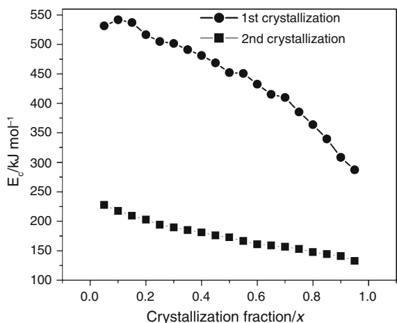
Fig. 9 Variation of the activation energy with the crystallization fraction of 35.5CaO–7.25La 2 O 3 –57.25B 2 O 3 glass for first and second crystallization events
