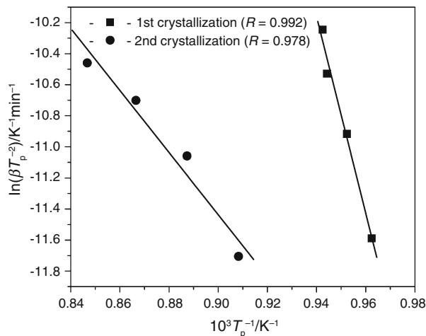
Fig. 3 \ln(\beta/T_p^2) vs. (1000/T_p) of 35.5CaO–7.25La 2 O 3 –57.25B 2 O 3 glass for first and second crystallization peaks
