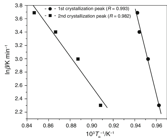
Fig. 5 \ln(\beta) vs. (1000/T_p) of 35.5CaO–7.25La 2 O 3 –57.25B 2 O 3 glass for first and second crystallization peaks
