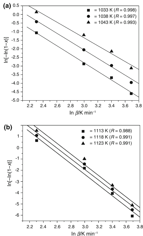
Fig. 7 \ln[-\ln(1-x)] vs. \ln \beta of 35.5CaO–7.25La 2 O 3 –57.25 B 2 O 3 glass for a first and b second crystallization peaks at different heating rates
