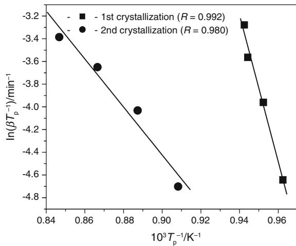
Fig. 4 \ln(\beta/T_p) vs. (1000/T_p) of 35.5CaO–7.25La 2 O 3 –57.25B 2 O 3 glass for first and second crystallization peaks
