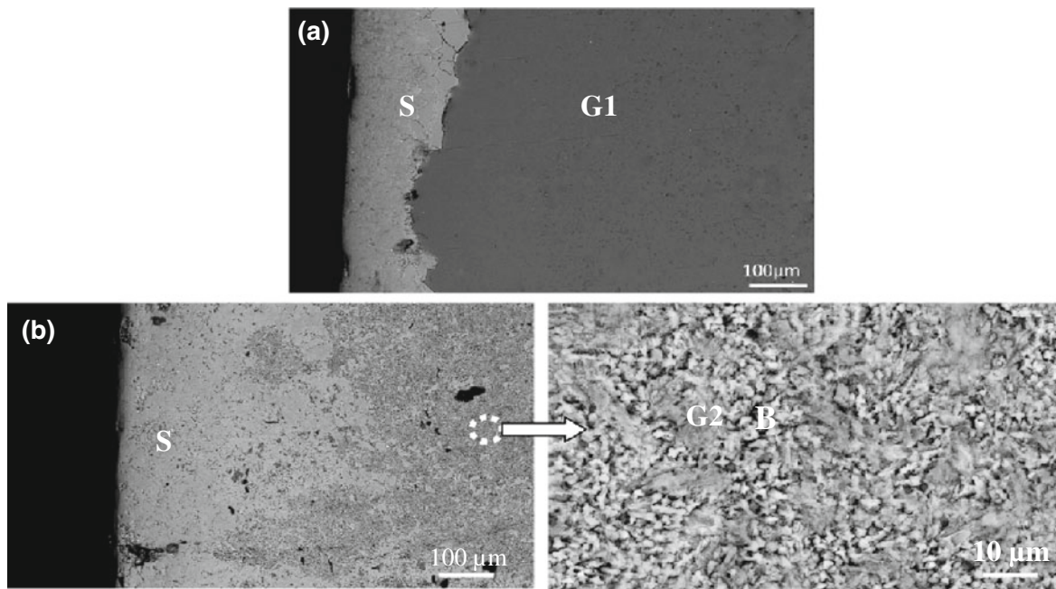
Fig. 10 FE-SEM micrographs showing the microstructure of 35.5CaO–7.25La 2 O 3 –57.25B 2 O 3 glasses ceramized at a 1043 K and b 1083 K for 30 min
