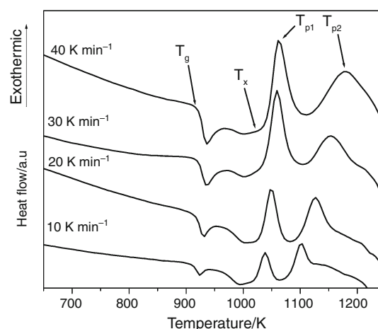
Fig. 1 DTA curves of 35.5\text{CaO}-7.25\text{La}_2\text{O}_3-57.25\text{B}_2\text{O}_3 glass at different heating rates
