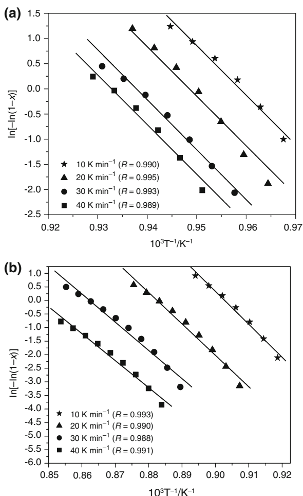
Fig. 8 \ln[-\ln(1-x)] vs. (1000/T) of 35.5\text{CaO}-7.25\text{La}_2\text{O}_3-57.25\text{B}_2\text{O}_3 glass for a first and b second crystallization peaks at different heating rates
