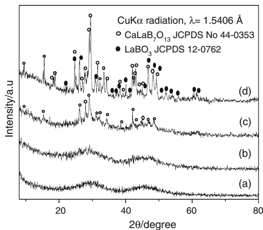
Fig. 2 X-ray diffraction patterns of a as-quenched of 35.5CaO–7.25La 2 O 3 –57.25B 2 O 3 glass and glasses ceramized at b 1013 K, c 1043 K, and d 1083 K for 30 min
