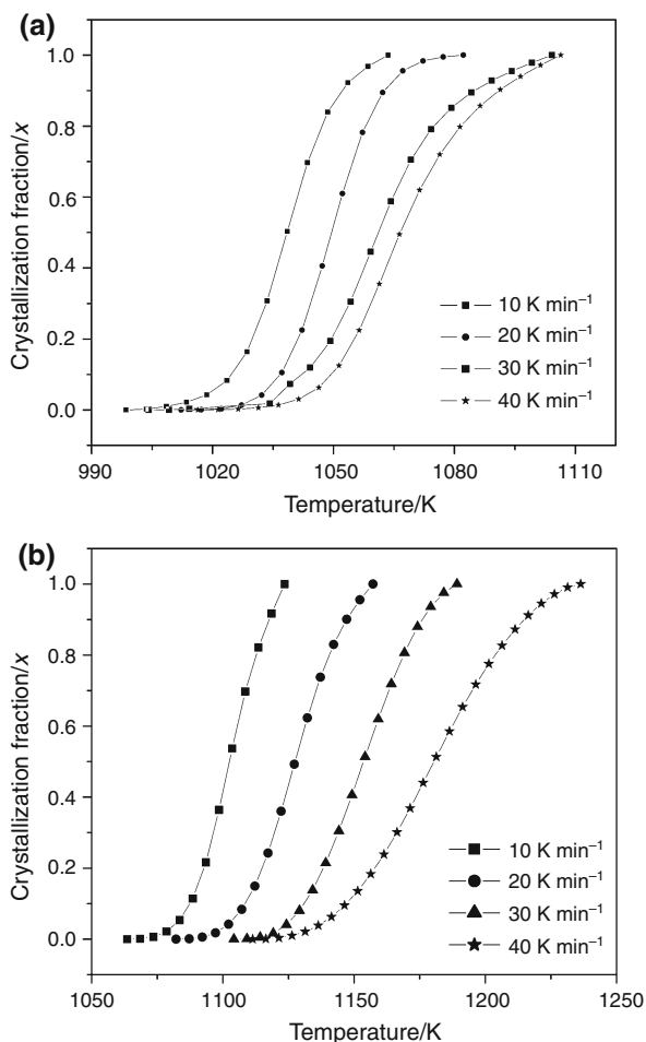
Fig. 6 The crystallization fraction vs. temperature of 35.5CaO–7.25La 2 O 3 –57.25B 2 O 3 glass for a first and b second crystallization peaks at different heating rates
